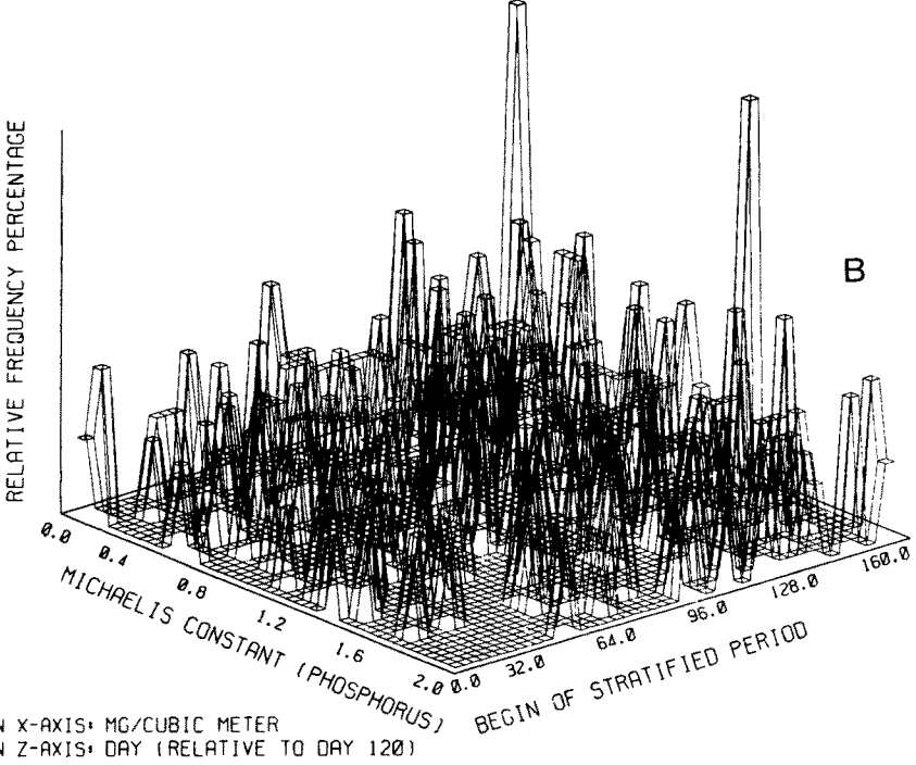
Fig. 4. Input-data space projections on planes of two input parameters; 293 data points, representing the sample inputvectors giving rise to the model response (empirical range) indicated in Fig. 1. Model response is sensitive to the input combination in (A), but not in (B)
