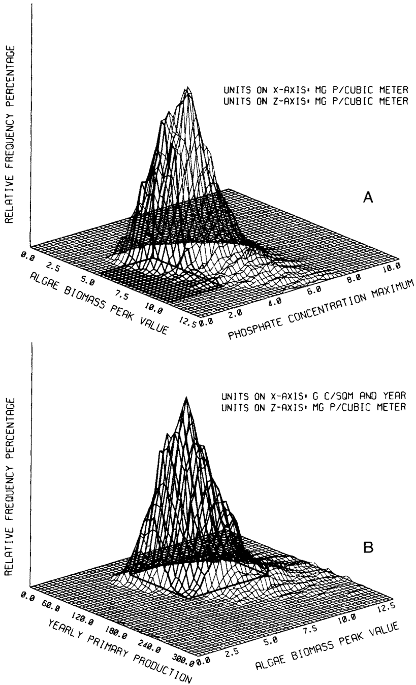
Fig. 3. Model response-space projections on planes of behaviour defining variables; 3000 model runs from a sub-region (80% of the single ranges, symmetric reduction) of the input-data space used for Fig. 2
