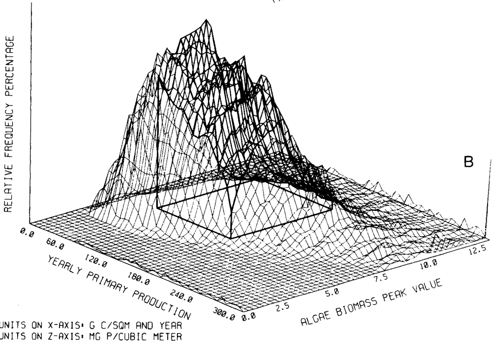
Fig. 2. Model response-space projections on planes of behaviour defining variables; 10 000 model runs over a field of "plausible" input-data ranges with rectangular probability density functions. The empirical, behaviour defining range is indicated by thicker lines and the projection rectangle in the x/z plane. The model used is based on the phosphorus/primary production model of Imboden & Gächter (1978); model response is sensitive to the behaviour defining ranges in (A), but less in (B)
