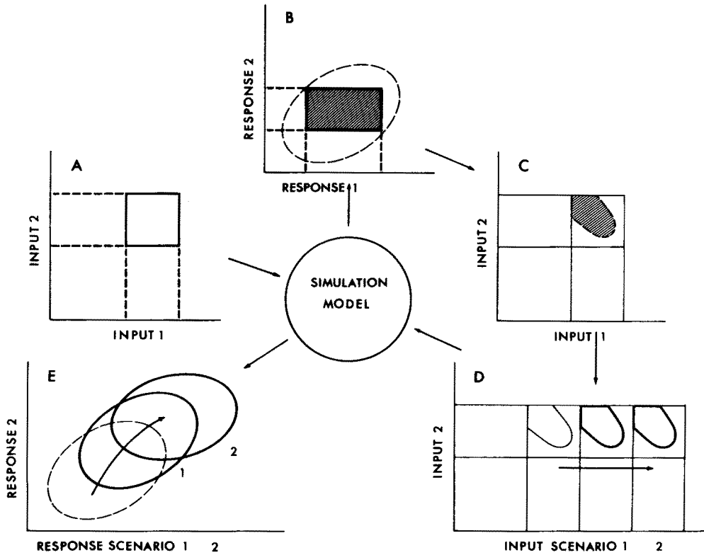
Fig. 1. Schematic summary of the approach, a two-dimensional example. (A) raw input-data space, defined by empirical ranges; (B) model response corresponding to A, indicating the empirical range of response patterns (compare Figs. 2, 3); (C) input-data space sub-region corresponding to the empirical range in B (compare Fig. 4); (D) Input scenarios, representing e.g. management alternatives; (E) model response to D (compare Fig. 5)
